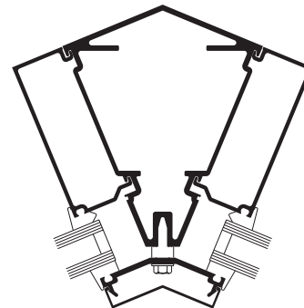
INSIDE 135° CORNER
