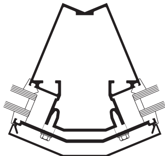
OUTSIDE 135° CORNER
