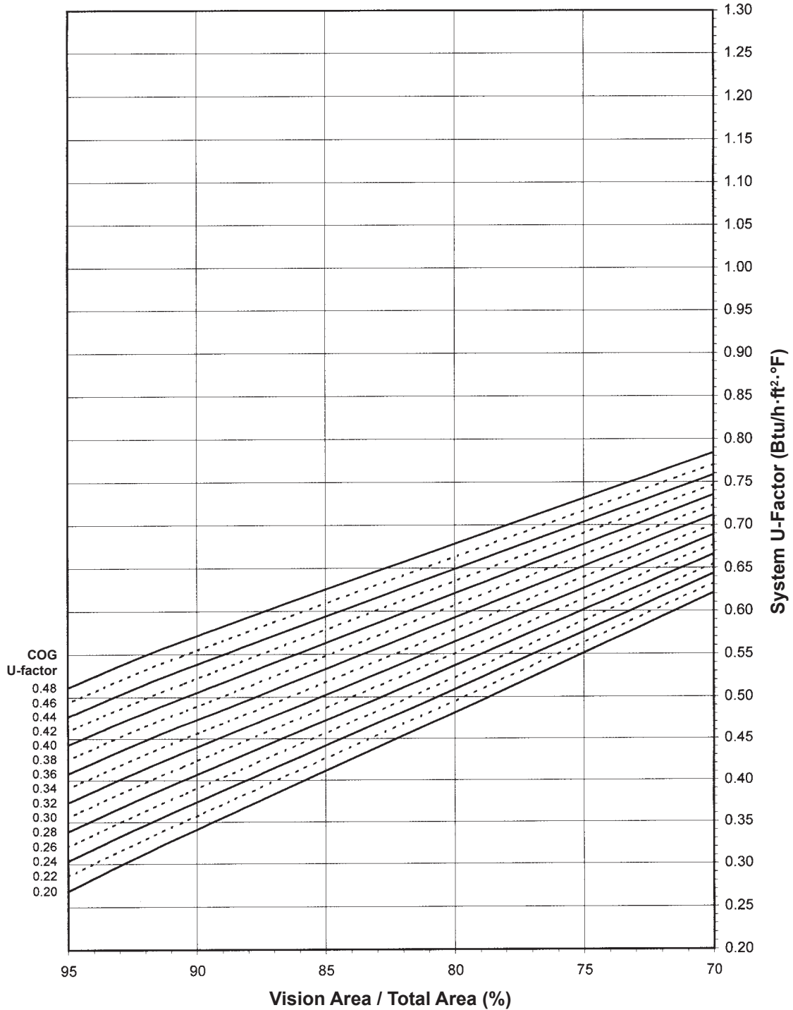
System U-Factor for Vision Glass
