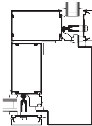
OUTSIDE 90° CORNER
