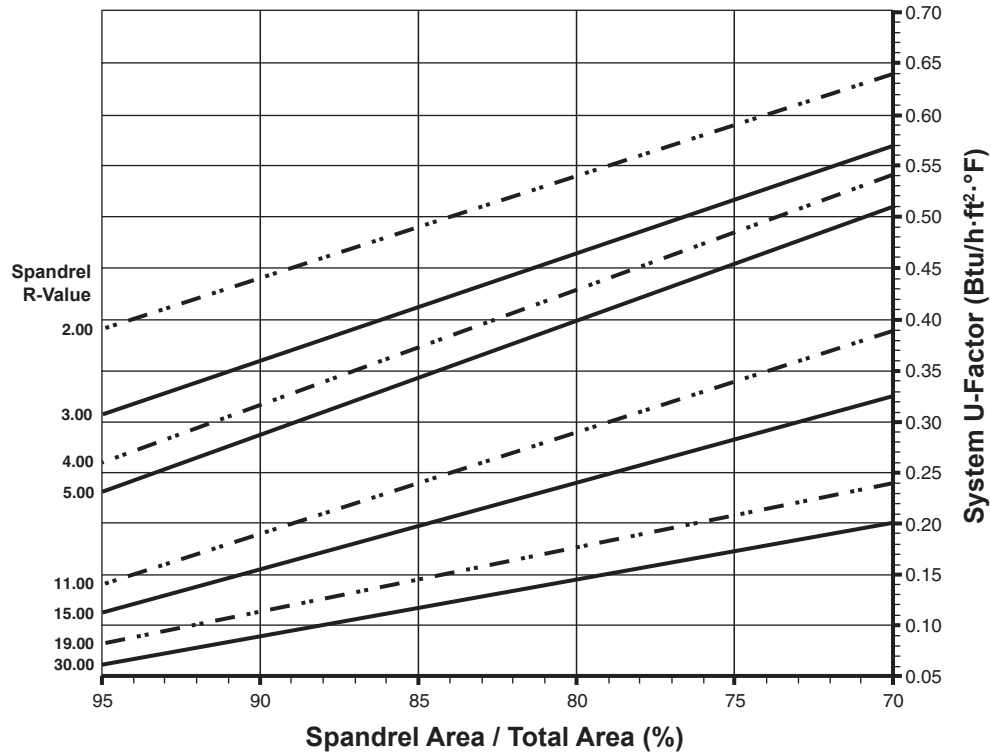
System U-Factors for Spandrel Glass
