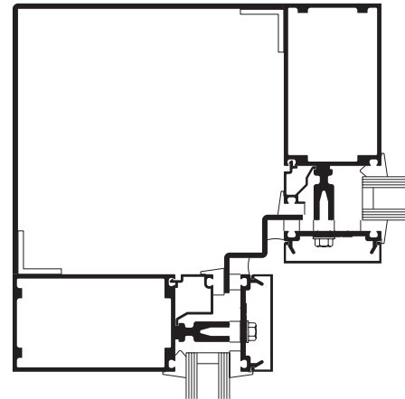
INSIDE 90° CORNER
